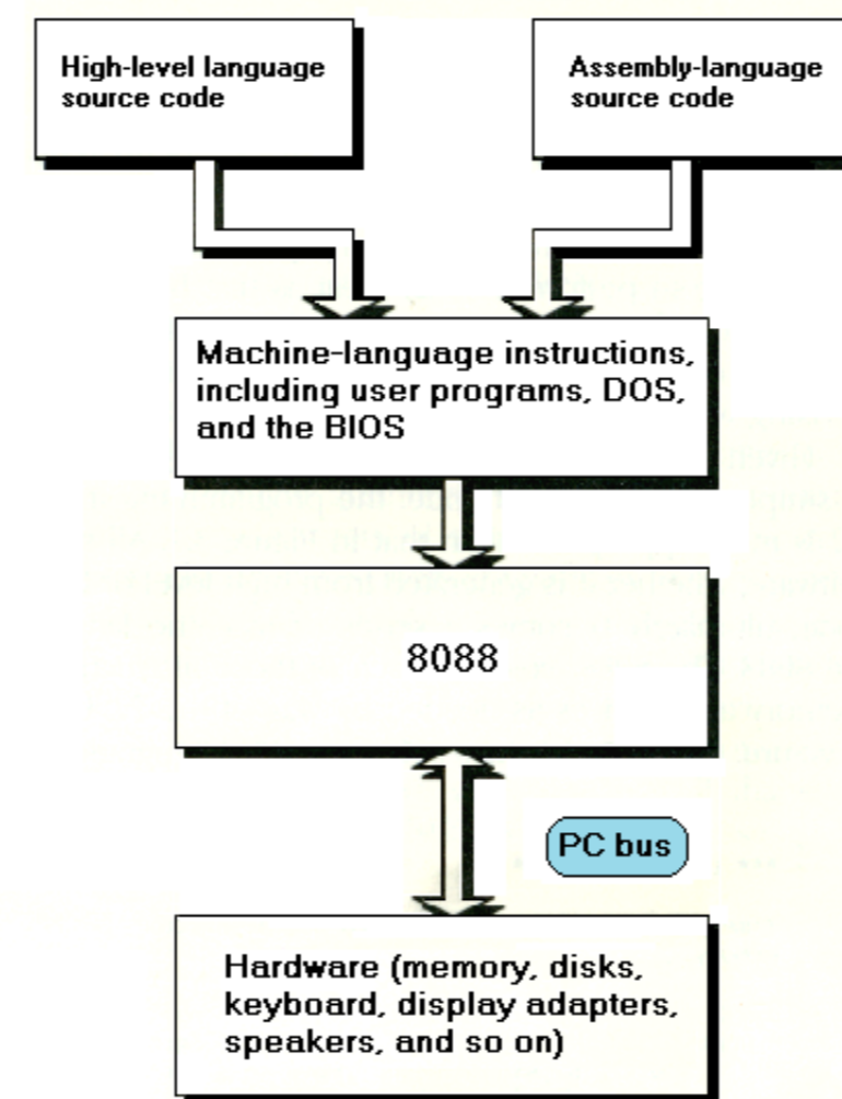
FIGURE 3.2 For high performance assembler programming, this view of the PC's resources is more useful than that of layered system software. Here the emphasis is on the interaction between machine language instructions, the 8088, and the hardware, with cycle eaters potentially present in the PC's hardware and bus.
